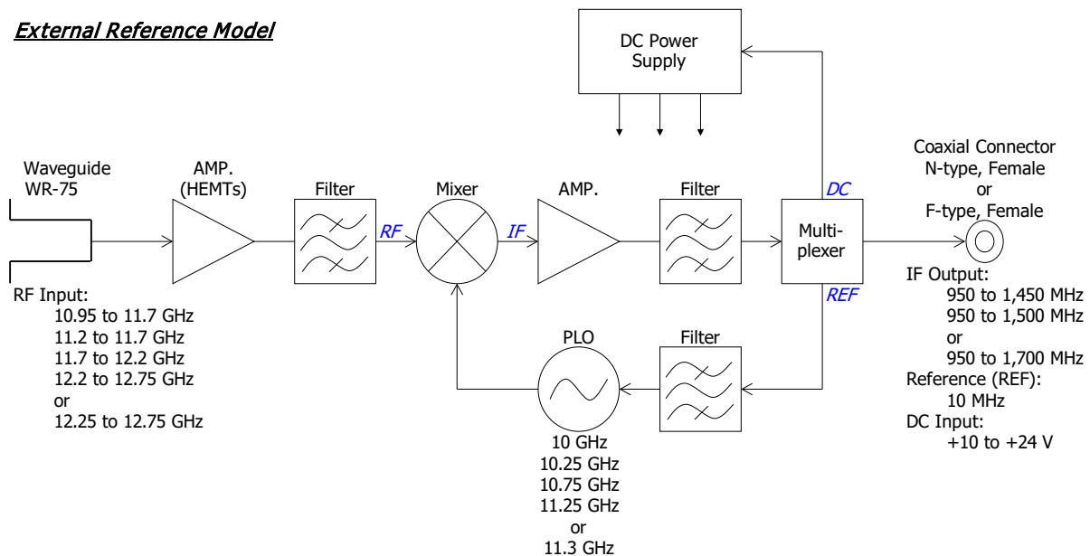
Fig.2 Functional Block Diagram
